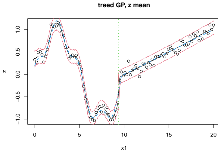
Figure 8: Posterior predictive distribution using btgp on synthetic sinusoidal data: mean and 90% pointwise credible interval, and MAP partition ( \hat{\mathcal{T}} ). The true mean is overlaid with a dashed line.
