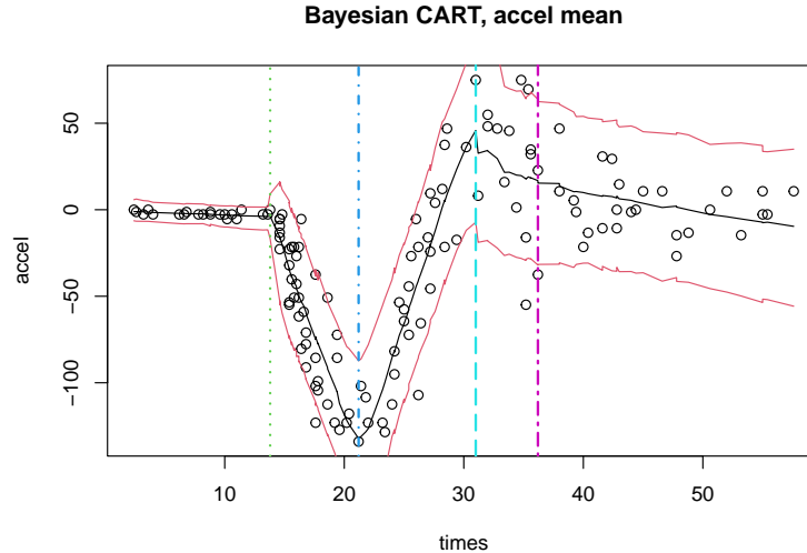
Figure 14: Posterior predictive distribution using bt1m on the motorcycle accident data: mean and 90% credible interval
